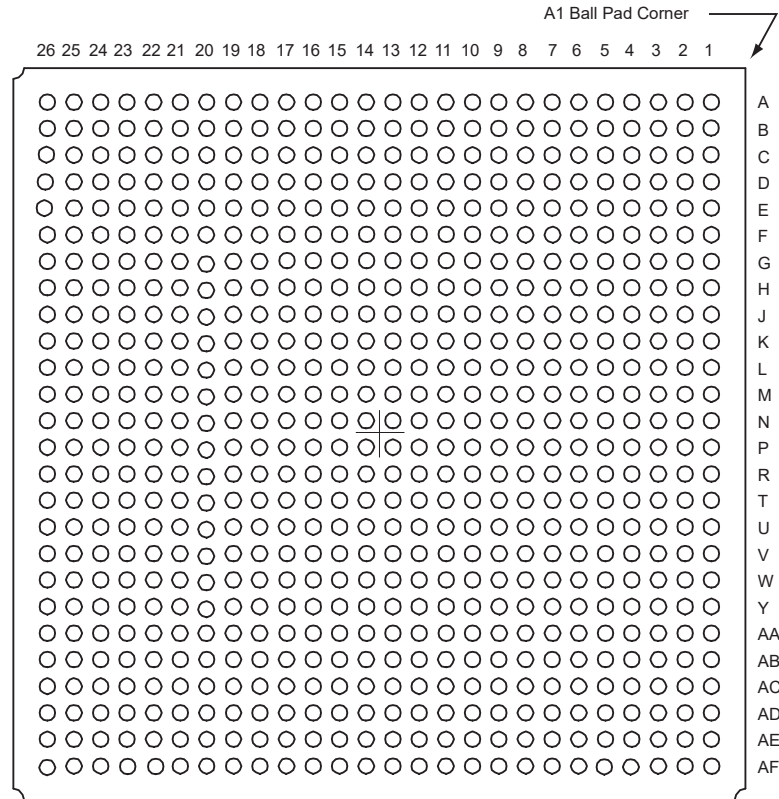
Figure 3-5. Package Bottom-View
