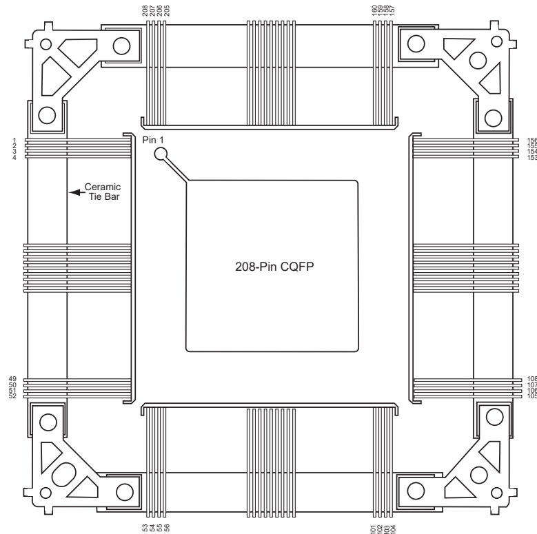
Figure 3-9. Package Bottom-View
