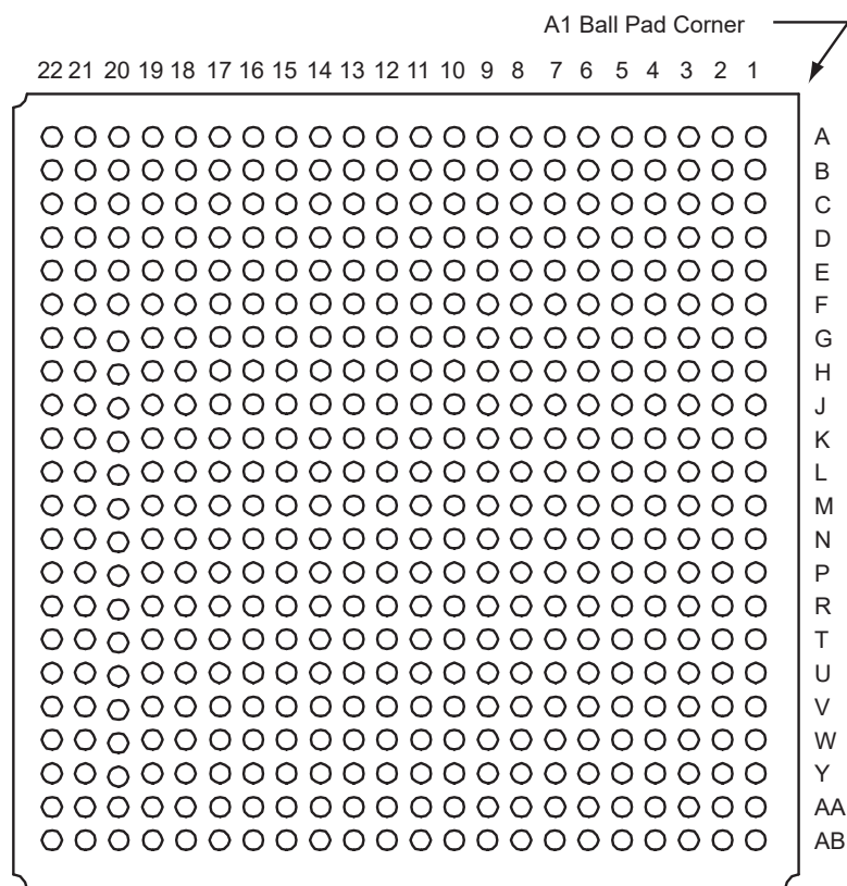
Figure 3-4. Package Bottom-View
