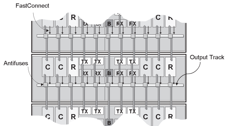
Figure 2-38. FastConnect Routing
