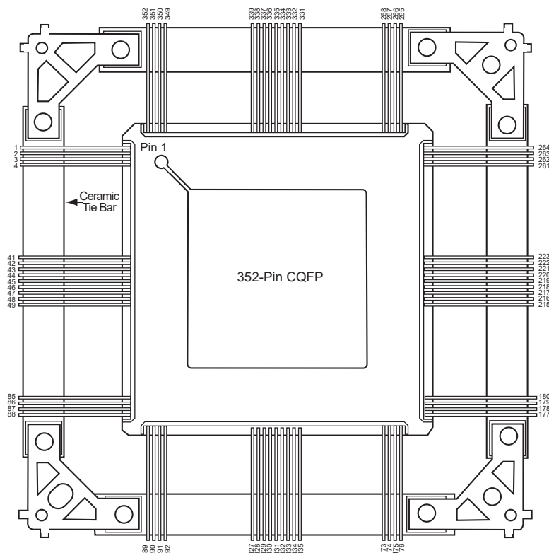
Figure 3-11. Package Bottom-View
