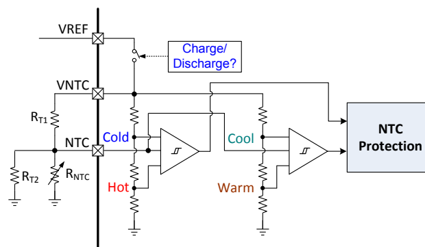
Figure 8: NTC Protection Circuit
