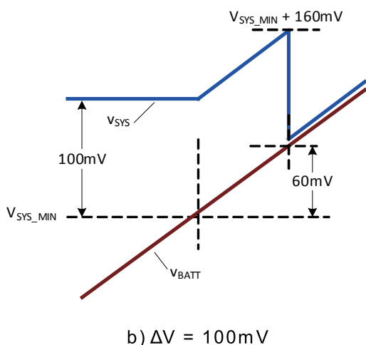
Figure 3: V_{SYS} Variation with V_{BATT}
