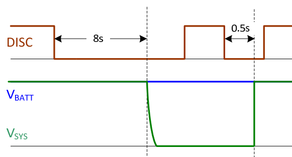
Figure 13: DISC Control Function
