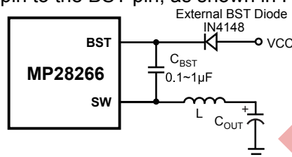
Figure 6: Optional External Bootstrap Diode for Enhanced Efficiency
