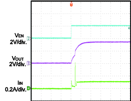
Inrush Current
