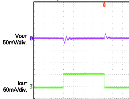
Load Transient
