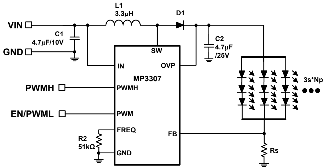
Figure 2: Typical Application for 3s \cdot N_p LEDs
