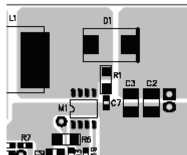
Figure 4—Layout Consideration
