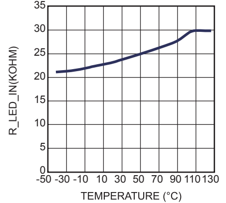
R VLED vs. Temperature
