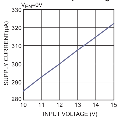
Supply Current, Output Disable vs. Input Voltage V_{EN}=0\text{V}
