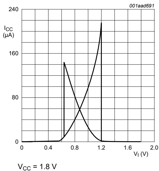
Fig. 12. Typical transfer characteristics
