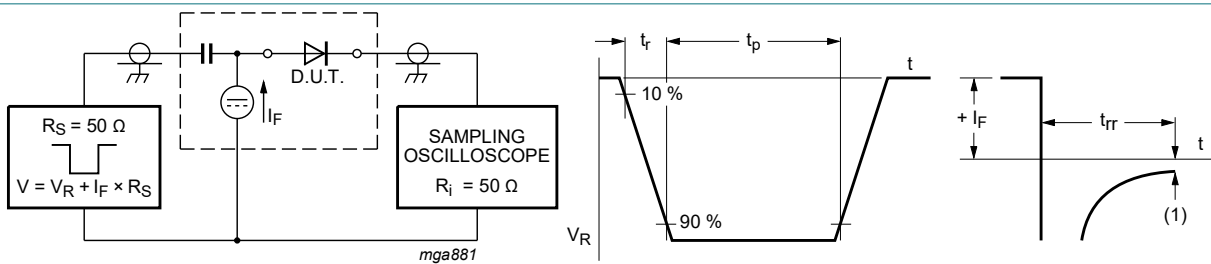
Fig. 6. Reverse recovery time test circuit and waveforms
