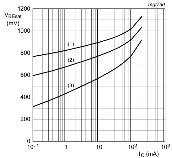
Fig. 9. BC846BQC-Q: Base-emitter voltage as a function of collector current; typical values
