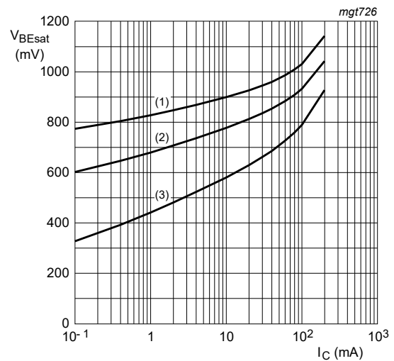
Fig. 5. BC846AQC-Q: Base-emitter voltage as a function of collector current; typical values
