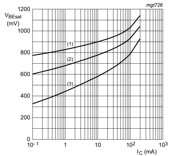
Fig. 3. BC847A-Q: Base-emitter voltage as a function of collector current; typical values
