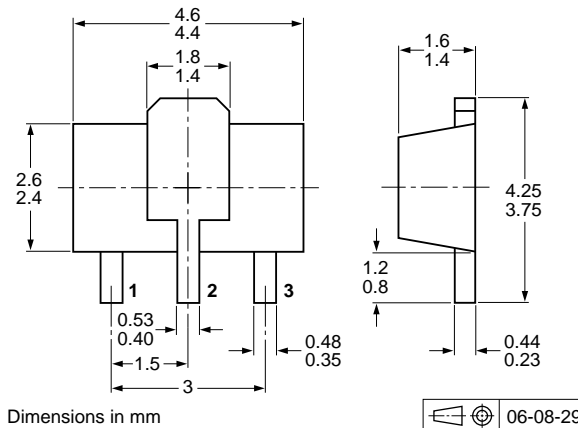
Fig 20. Package outline SOT89 (SC-62/TO-243)
