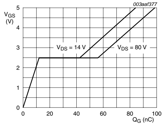
Fig 16. Gate-source voltage as a function of gate charge; typical values
