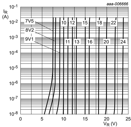
Fig. 9. Reverse current as a function of reverse voltage; typical values (BZX84J-B/C7V5 to B/C24)
