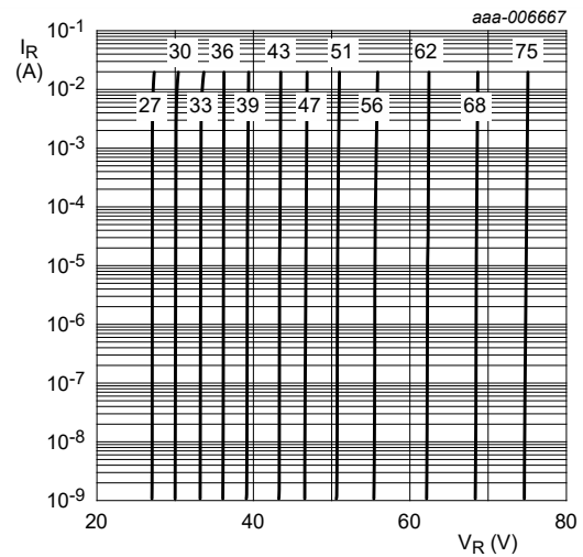
Fig. 10. Reverse current as a function of reverse voltage; typical values (BZX84J-B/C27 to B/C75)
