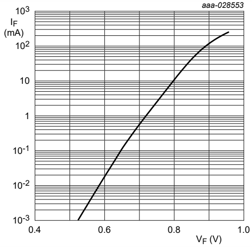
Fig. 5. Forward current as a function of forward voltage; typical values (BZX84J-B/C75)
