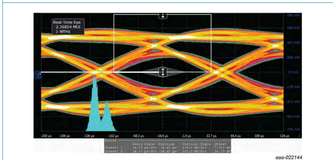
Fig 11. HDMI 2.0 eye diagram TP2, test board with PCMF2USB30; typical values
