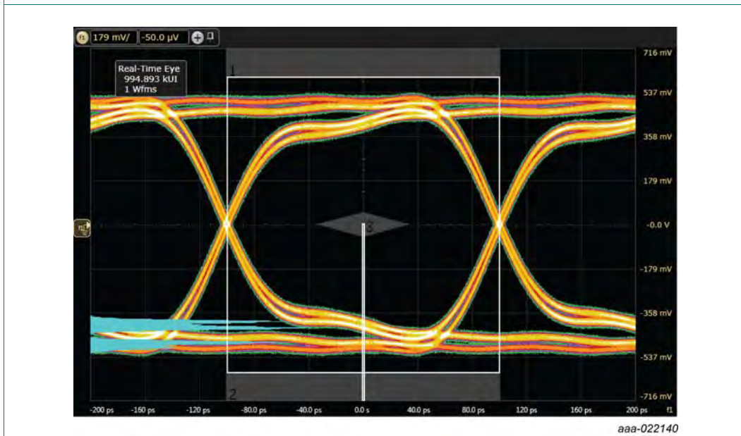
Fig 7. USB 3.1 eye diagram, test board with PCMF2USB30; typical values
