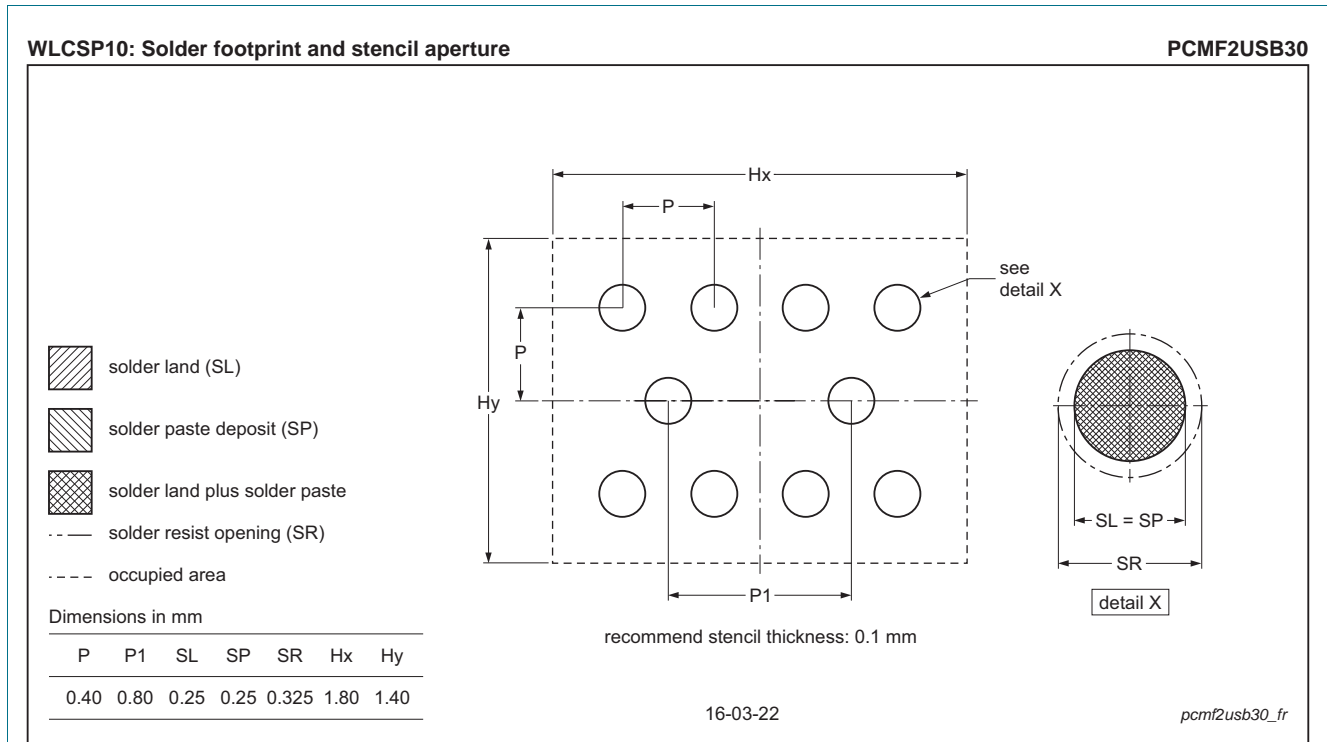
Fig 28. Soldering footprint WLCSP10 (PCMF2USB30)
