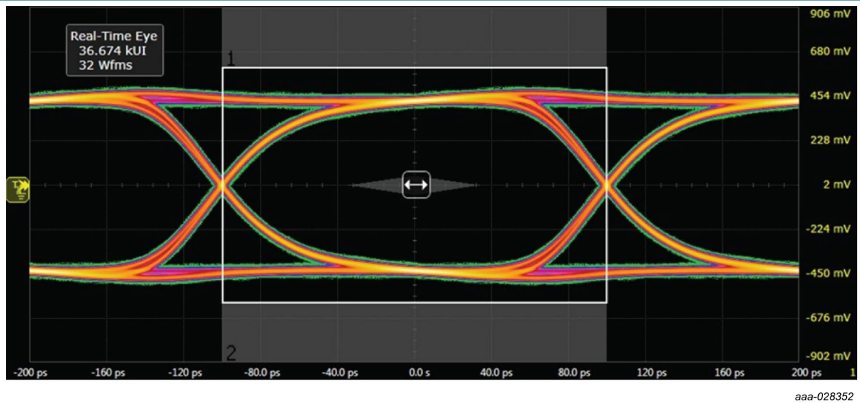
Fig. 8. USB 3.2 eye diagram 5 Gbps, test board without device; typical values
