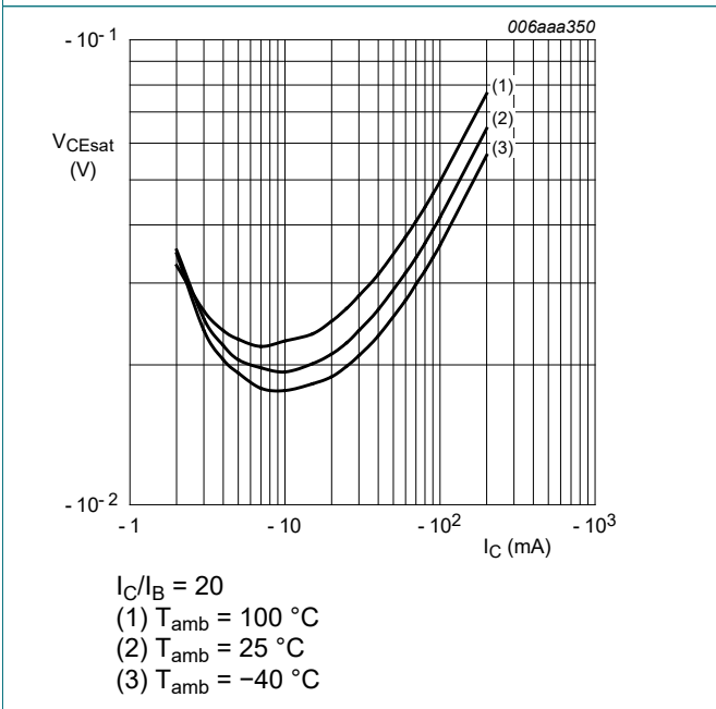
Fig. 9. TR2 (PNP): Collector-emitter saturation voltage as a function of collector current; typical values
