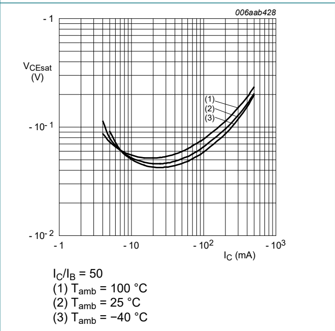
Fig. 10. TR2 (PNP): Collector-emitter saturation voltage as a function of collector current; typical values
