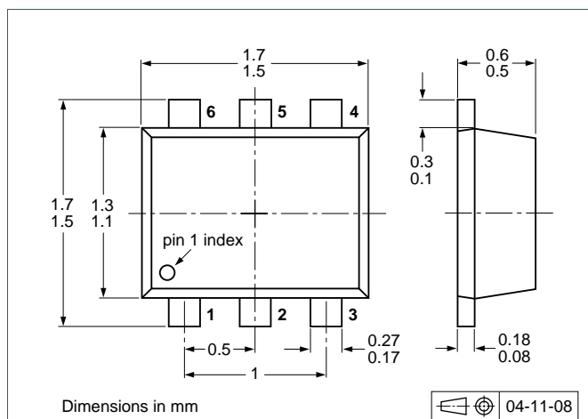
Fig 16. Package outline PEMD12 (SOT666)
