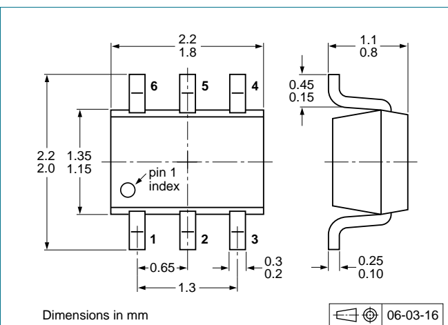
Fig 17. Package outline PUMD12 (SOT363)
