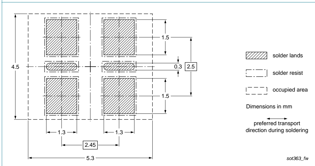
Fig 20. Wave soldering footprint PUMD12 (SOT363)
