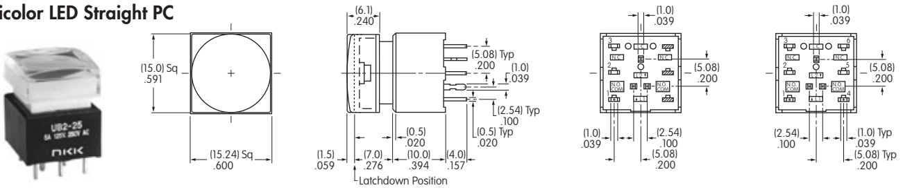
UB225SKG03CF-1JB
