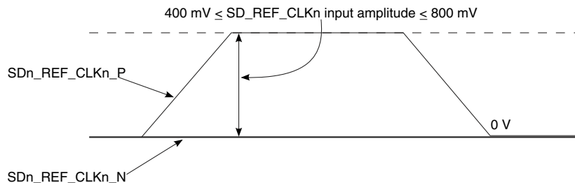
Figure 71. Single-ended reference clock input DC requirements
