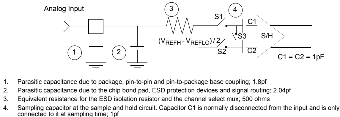
Figure 10-24 Equivalent Circuit for A/D Loading
