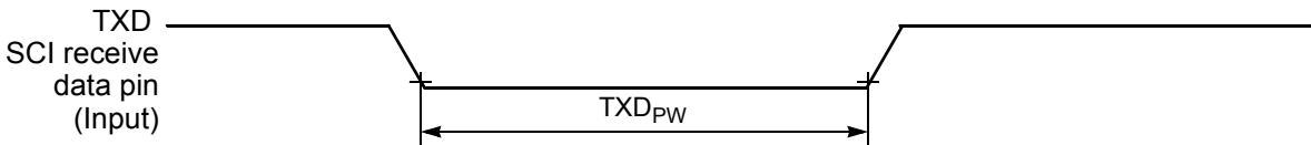
Figure 10-18 TXD Pulse Width
