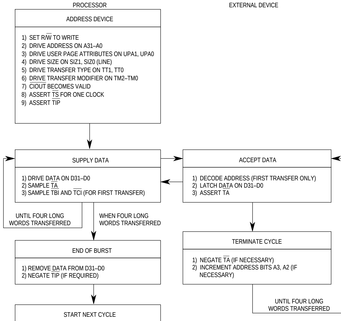
Figure 7-16. Line Write Transfer Flowchart
