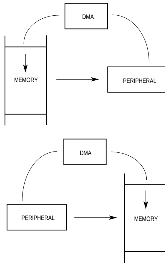
Figure 6-2. Single-Address Transfers
