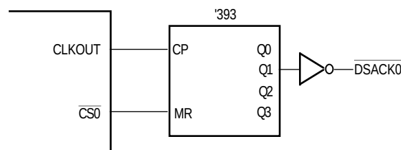
Figure 10-8. External Circuitry for 8-Bit Boot ROM
