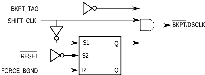
Figure 5-26. BKPT/DSCLK Logic Diagram
