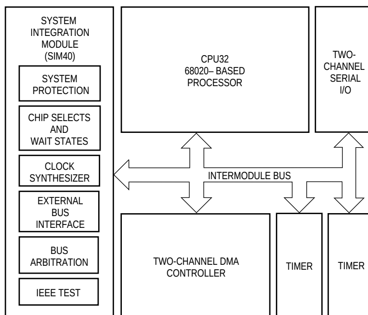
Figure 1-1. Block Diagram
