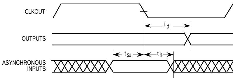
Figure 10-11. Signal Relationships to CLKOUT
