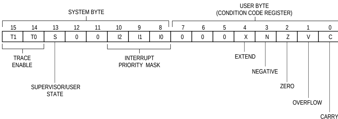
Figure 5-5. Status Register
