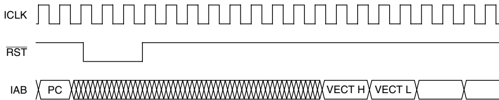
Figure 7-4. External Reset Timing
