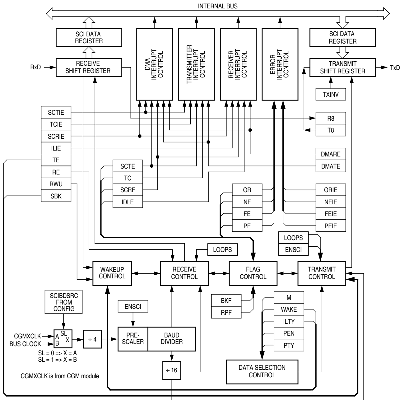
Figure 11-2. SCI Module Block Diagram
