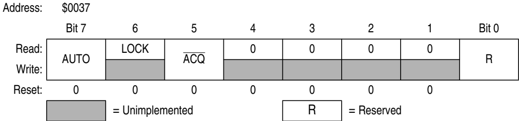
Figure 6-5. PLL Bandwidth Control Register (PBWCR)
