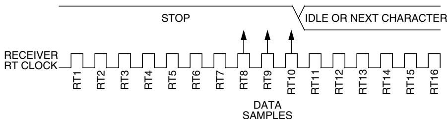
Figure 12-11. Fast Data
