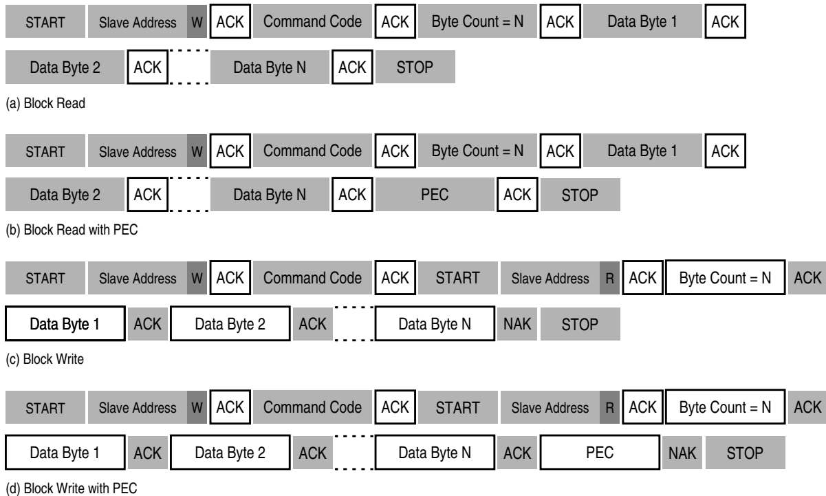
Figure 14-19. Block Read/Write
