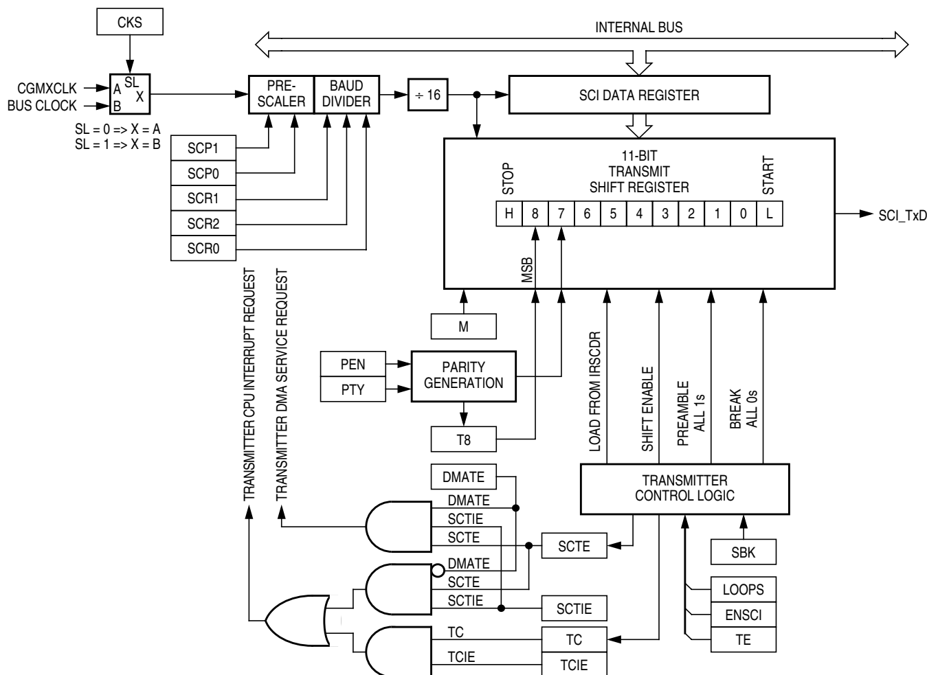
Figure 12-7. SCI Transmitter
