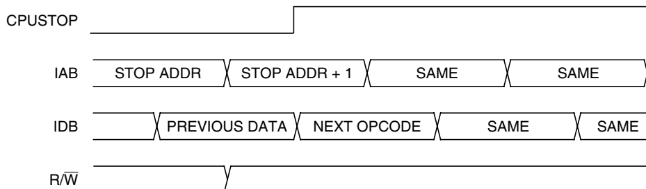
Figure 7-18. Stop Mode Entry Timing
