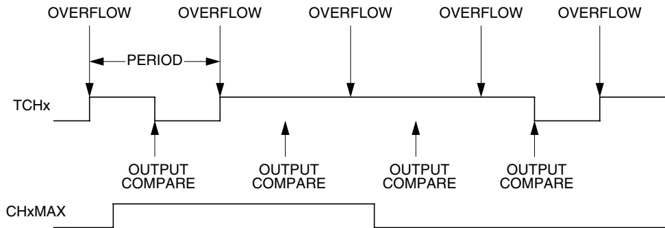
Figure 9-11. CHxMAX Latency
