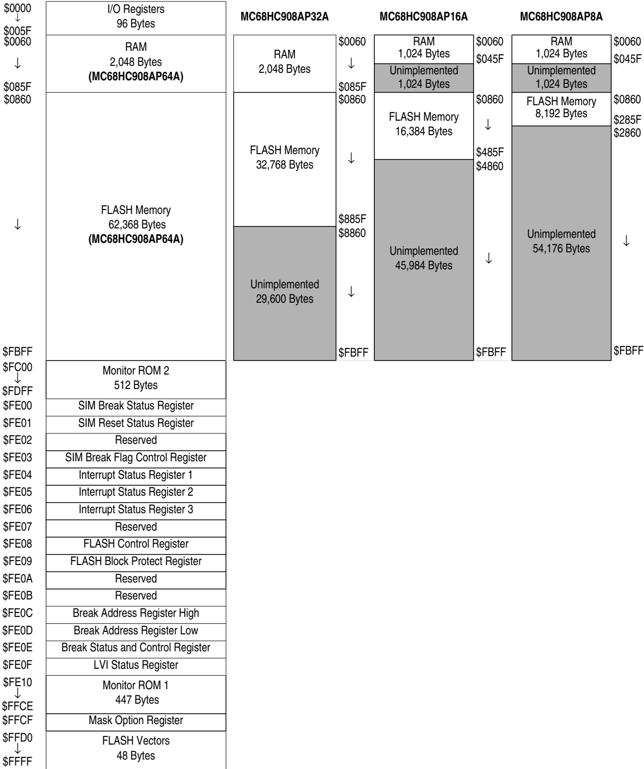
Figure 2-1. Memory Map
