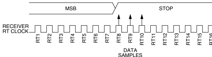
Figure 12-10. Slow Data
