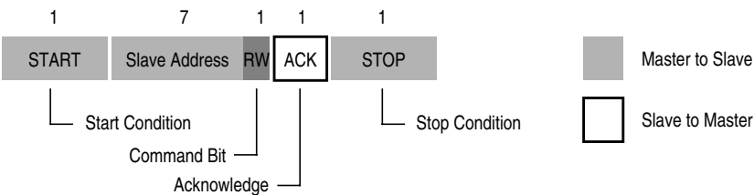
Figure 14-13. Quick Command
