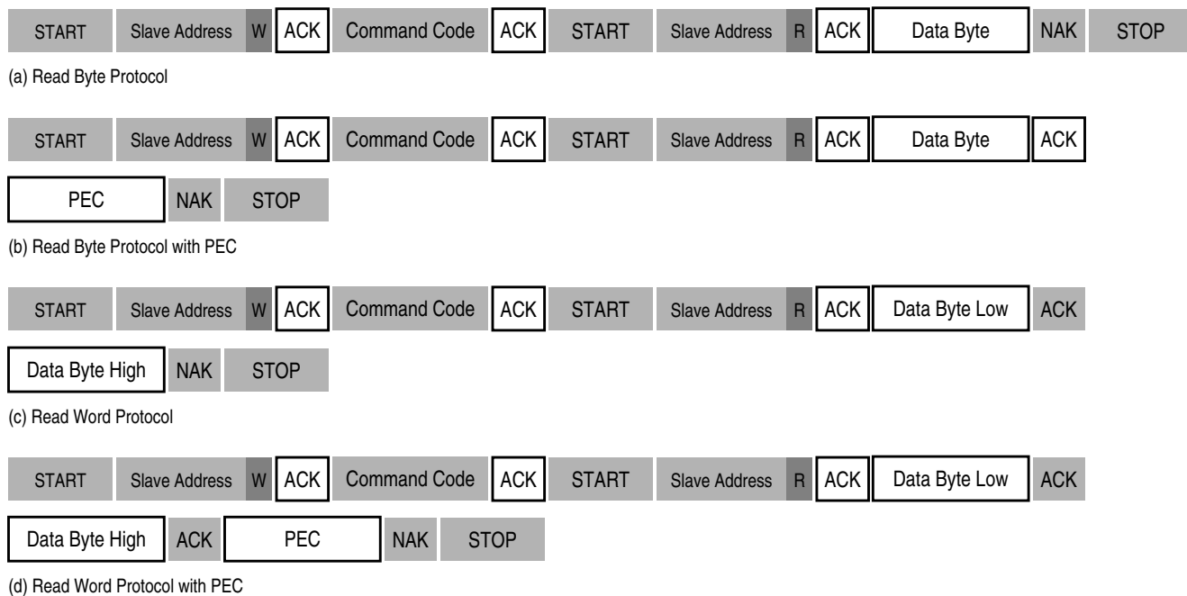
Figure 14-17. Read Byte/Word
