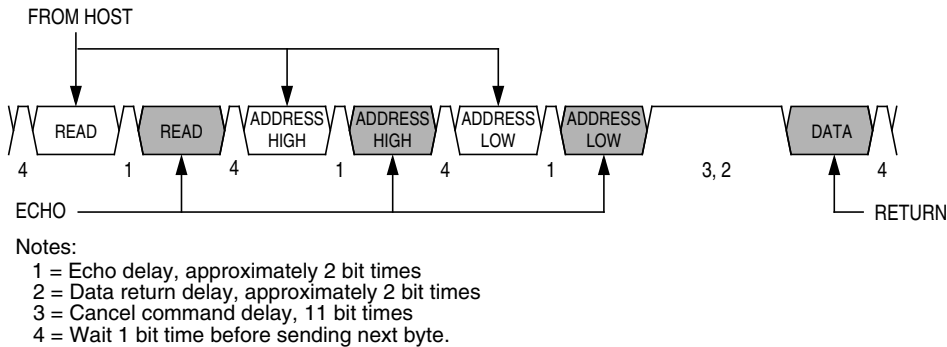
Figure 8-5. Read Transaction
