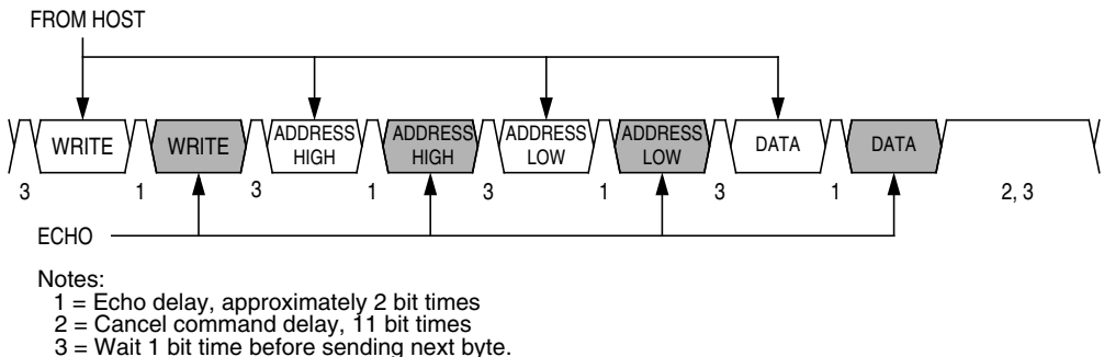
Figure 8-6. Write Transaction
