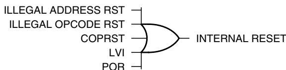
Figure 7-6. Sources of Internal Reset
