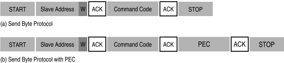
Figure 14-14. Send Byte
