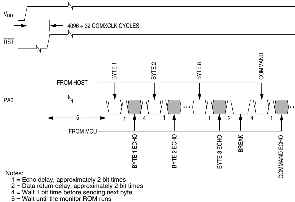
Figure 19-17. Monitor Mode Entry Timing
