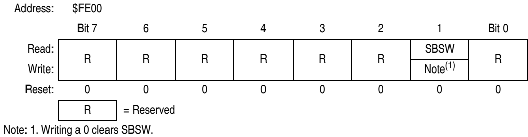
Figure 15-20. SIM Break Status Register (SBSR)
