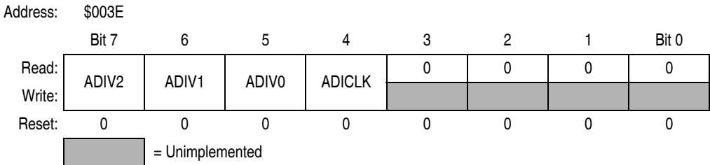
Figure 3-5. ADC Clock Register (ADCLK)
