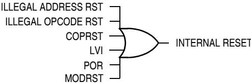
Figure 15-6. Sources of Internal Reset
