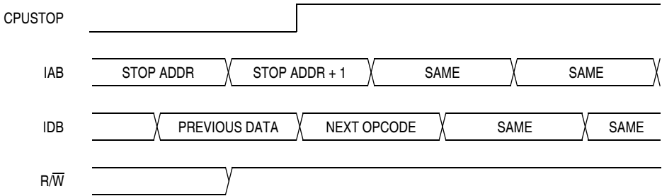
Figure 15-18. Stop Mode Entry Timing
