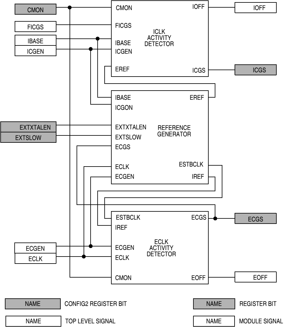
Figure 7-5. Clock Monitor Block Diagram
