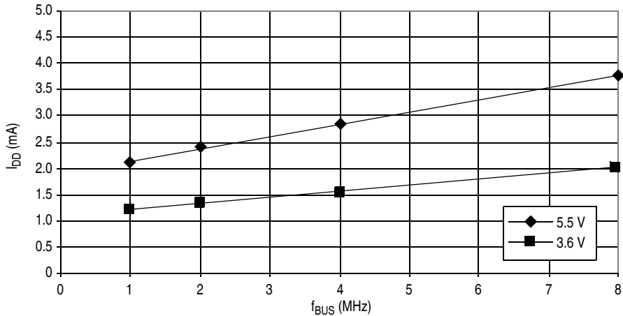
Figure 20-16. Typical Wait Mode I_{DD} , with all Modules Disabled ( -40^{\circ}\text{C} to 85^{\circ}\text{C} )
