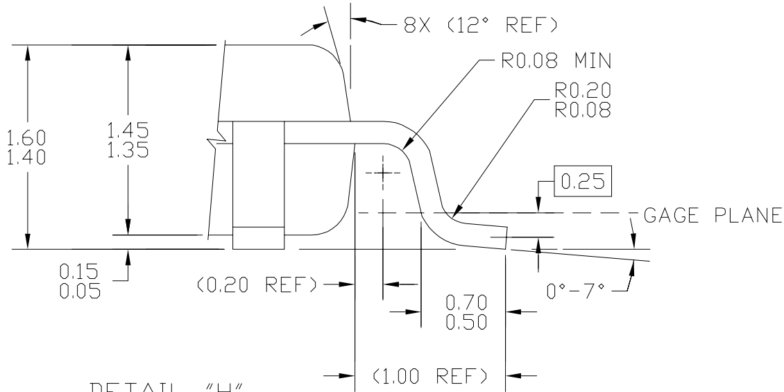
DETAIL "H"
