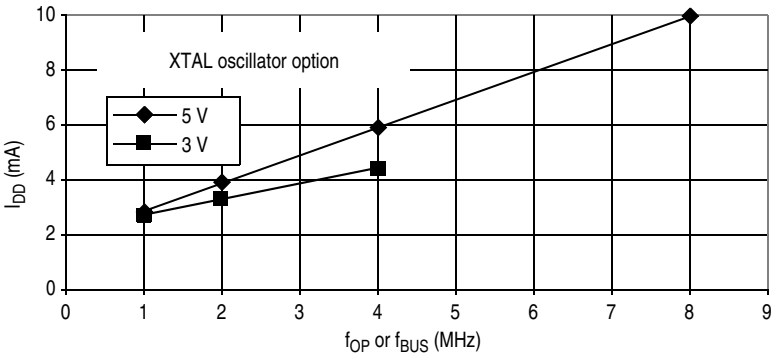
Figure 17-5. Typical Operating I DD (XTAL osc), with All Modules Turned On (25°C)
