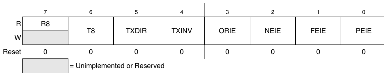
Figure 11-10. SCI Control Register 3 (SCIC3)
