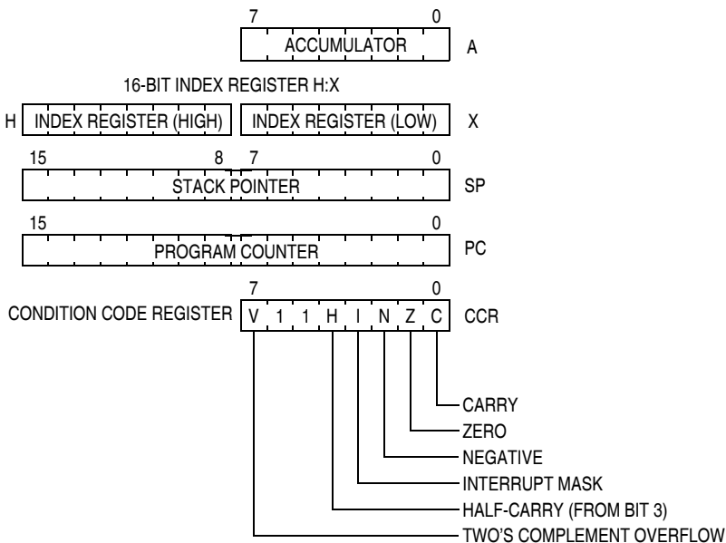
Figure 7-1. CPU Registers
