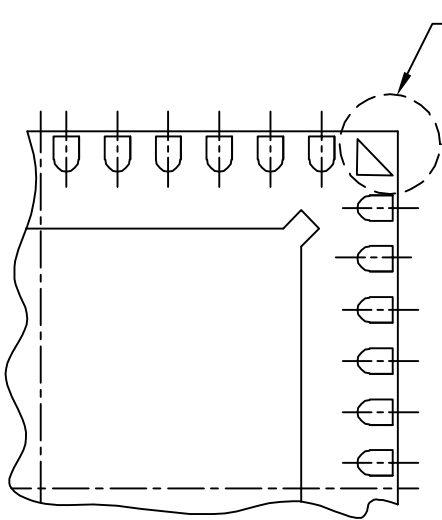
DETAIL M PIN 1 BACKSIDE IDENTIFIER OPTION
