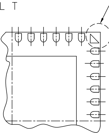
DETAIL M PIN 1 BACKSIDE IDENTIFIER OPTION
