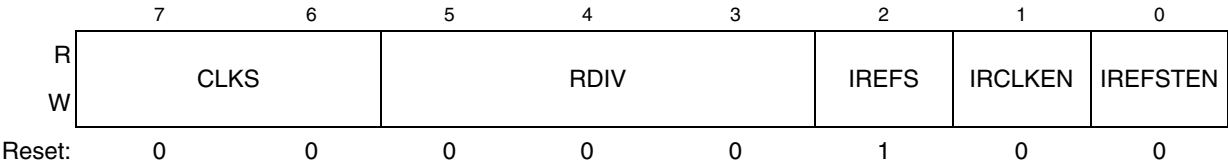
Figure 11-3. ICS Control Register 1 (ICSC1)
