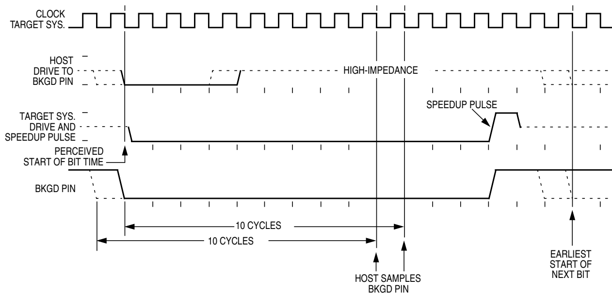
Figure 18-9. BDM Target-to-Host Serial Bit Timing (Logic 0)
