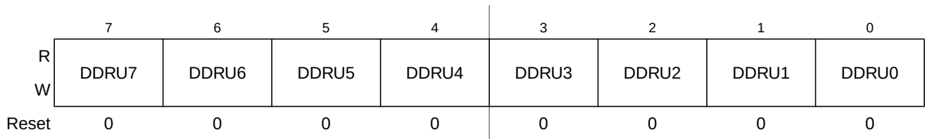
Figure 4-45. Port U Data Direction Register (DDRU)
