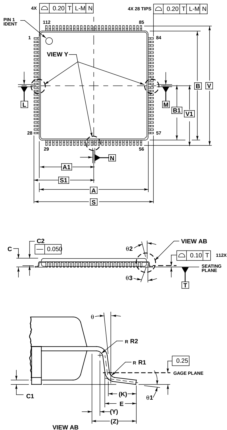
Figure C-1. 112-Pin LQFP Mechanical Dimensions (case no. 987)
