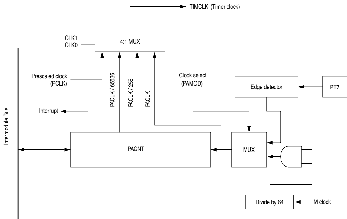
Figure 16-2. 16-Bit Pulse Accumulator Block Diagram
