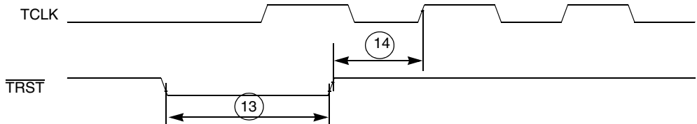
Figure 17. \overline{TRST} Timing
