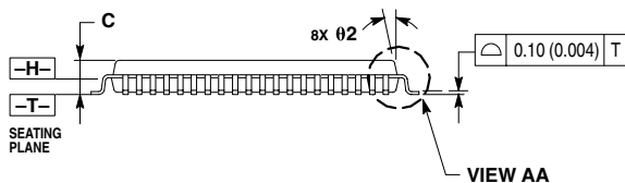
VIEW AA
