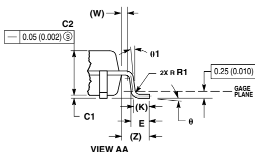
VIEW AA
