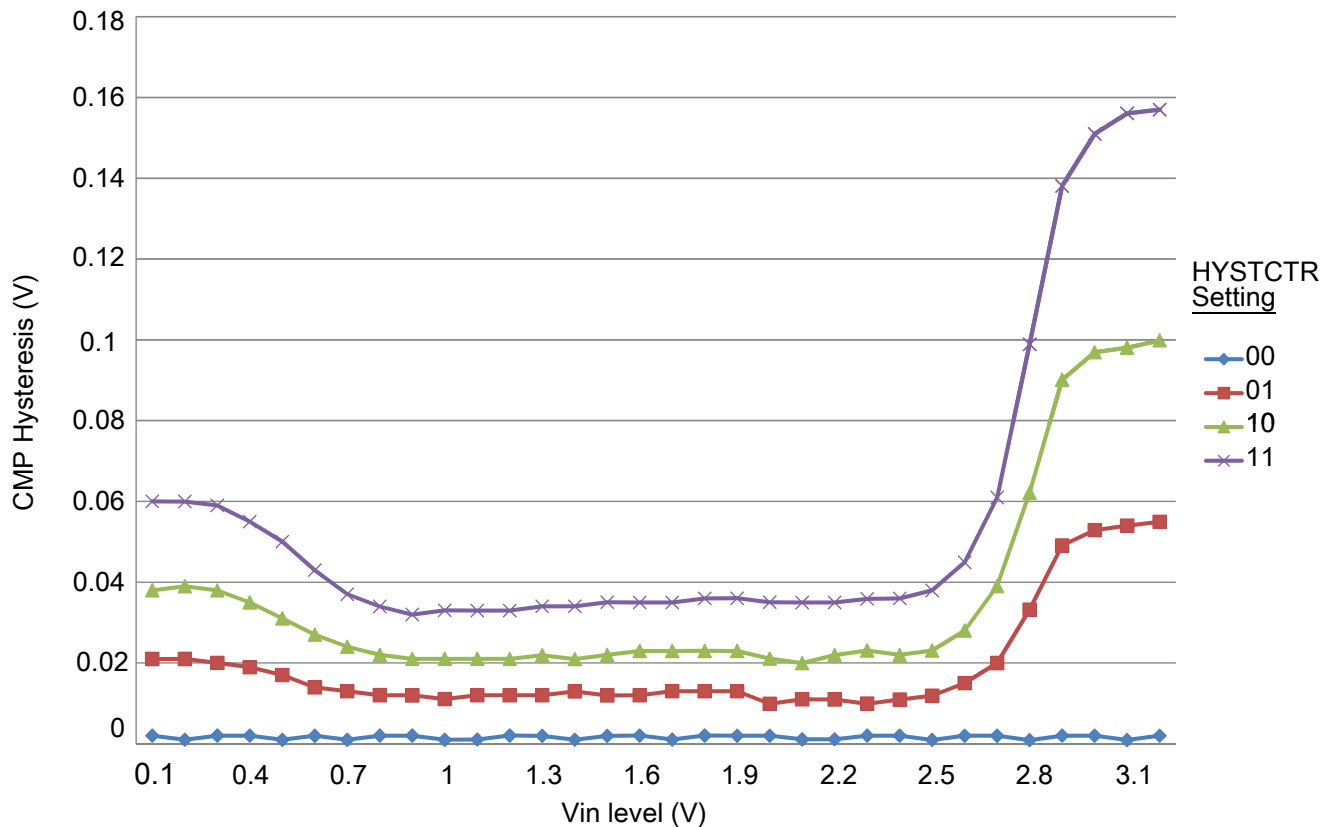
Figure 5. Typical hysteresis vs. Vin level (VDD = 3.3 V, PMODE = 1)
