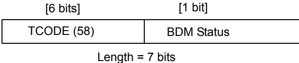
Figure 24-81. BDM Status Message Format
