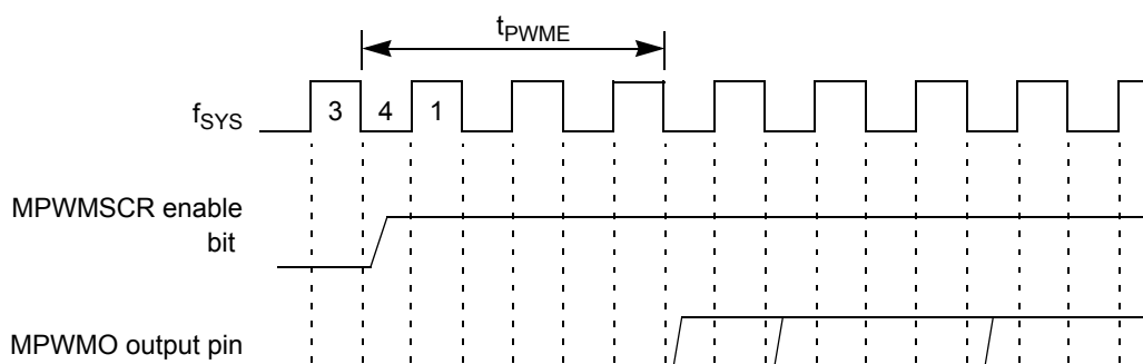
Figure F-50. MPWMSM Enable to MPWMO Output Pin Rising Edge Timing Diagram
