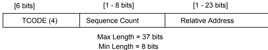
Figure 24-20. Indirect Branch Message Format
