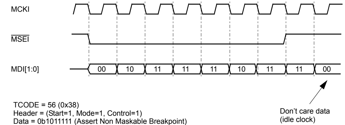
Figure 24-87. DSDI Data Message (Assert Non-Maskable Breakpoint)
