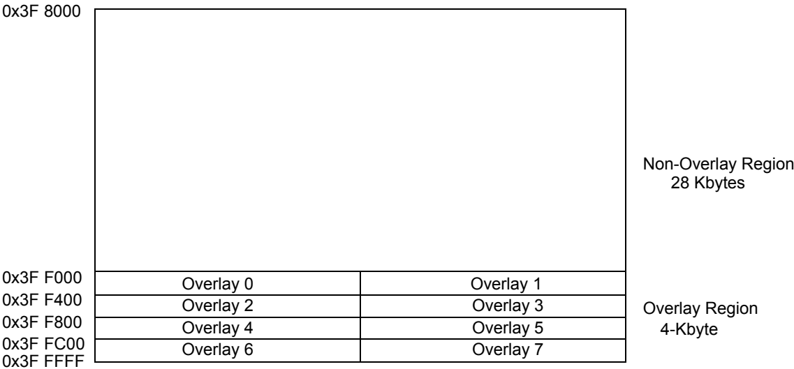
Figure 22-4. CALRAM Array
