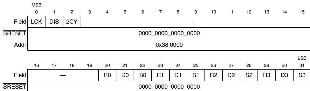
Figure 22-9. CALRAM Module Configuration Register (CRAMMCR)
