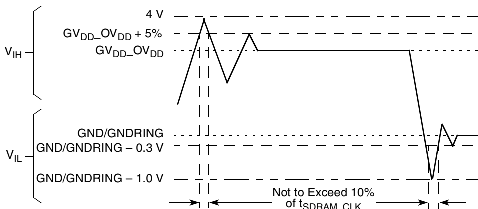
Figure 3. Overshoot/Undershoot Voltage
