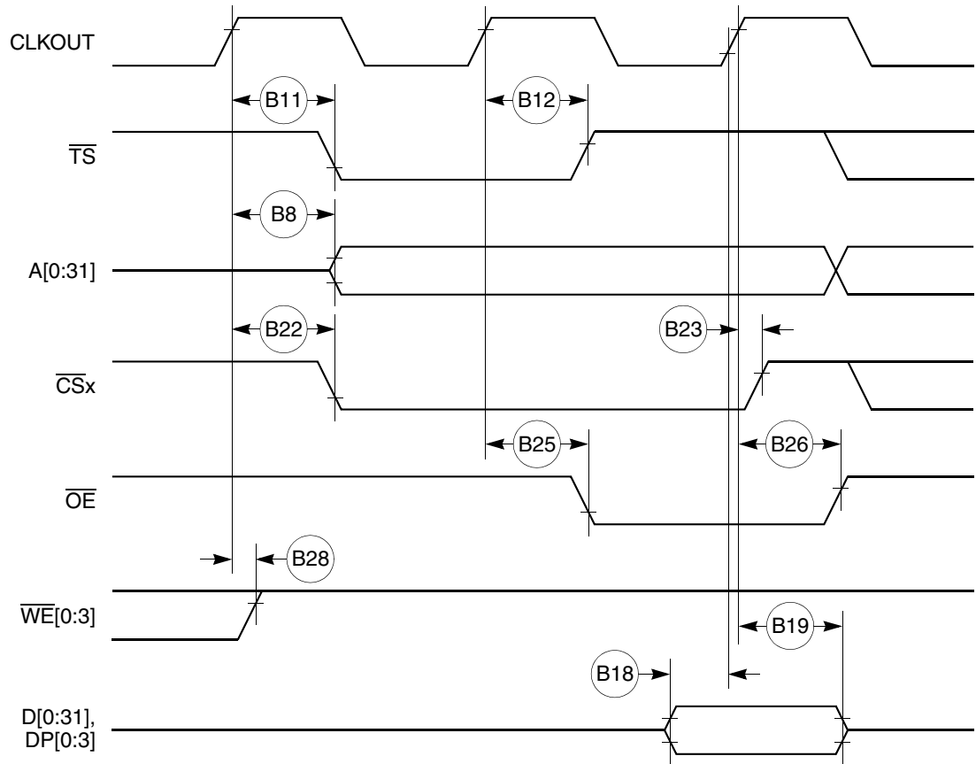
Figure 10. External Bus Read Timing (GPCM Controlled—ACS = 00)
