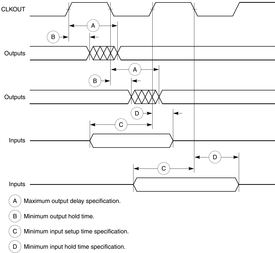
Figure 3. Control Timing
