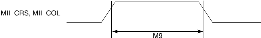
Figure 74. MII Async Inputs Timing Diagram
