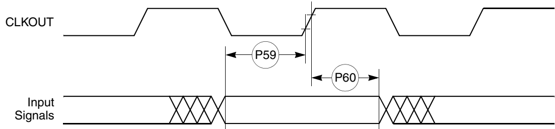
Figure 29. PCMCIA Input Port Timing
