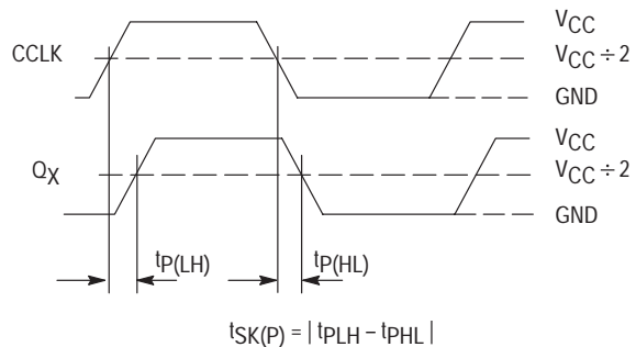
Figure 16. Output Pulse Skew (tSK(P)) Test Reference
