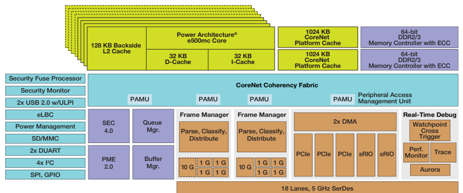
■ Core Complex (CPU, L2 and Frontside CoreNet Platform Cache) ■ P4080 and P4081 Only ■ Accelerators and Memory Control ■ Networking Elements ■ P4080 and P4040 Only ■ Basic Peripherals and Interconnect
