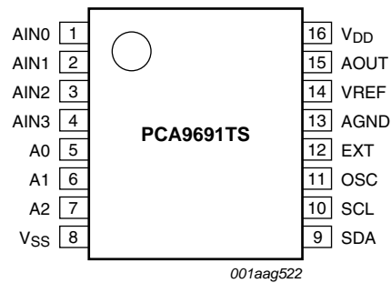
Fig 3. Pin configuration for TSSOP16 (PCA9691TS)
