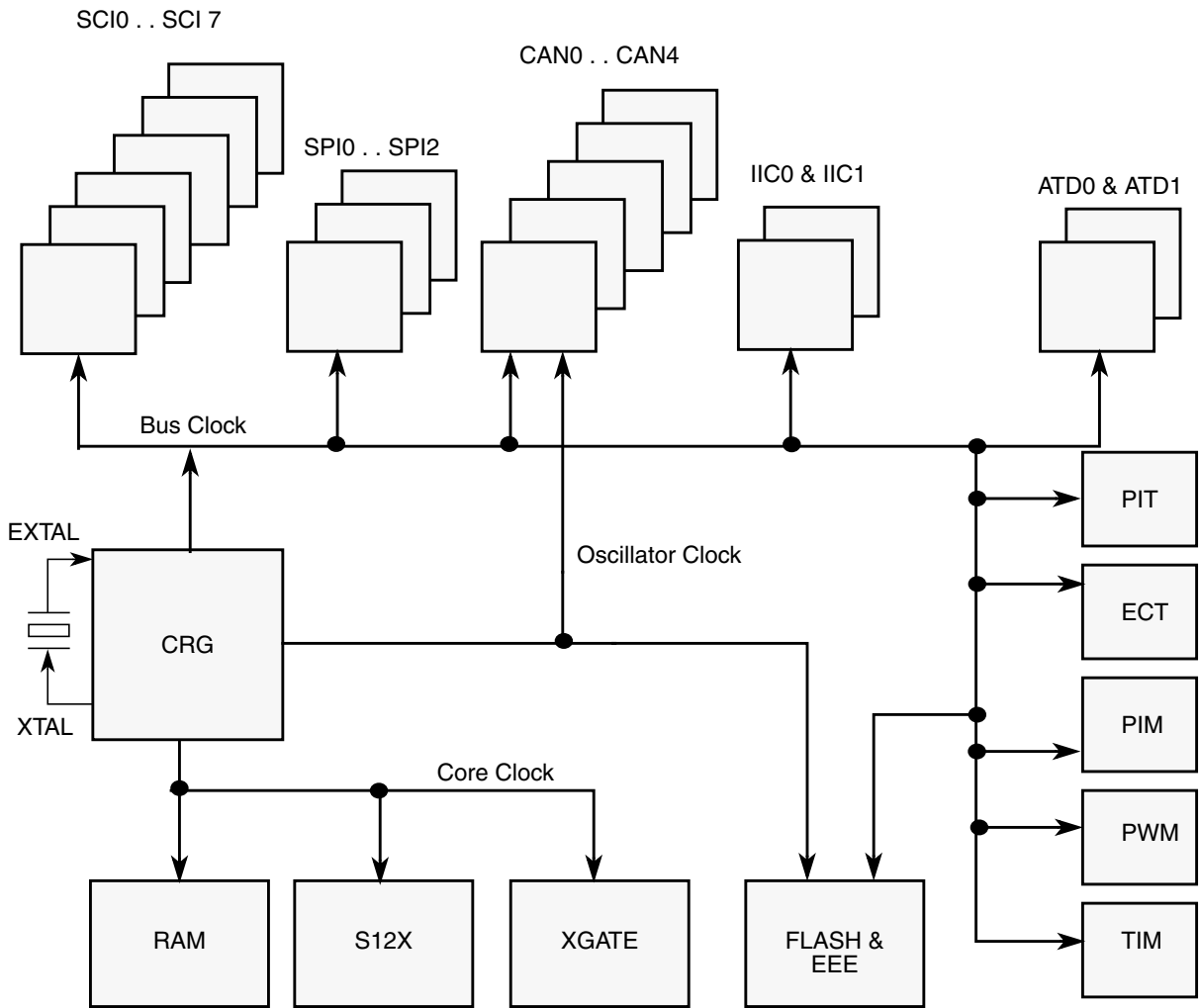
Figure 1-9. Clock Connections
