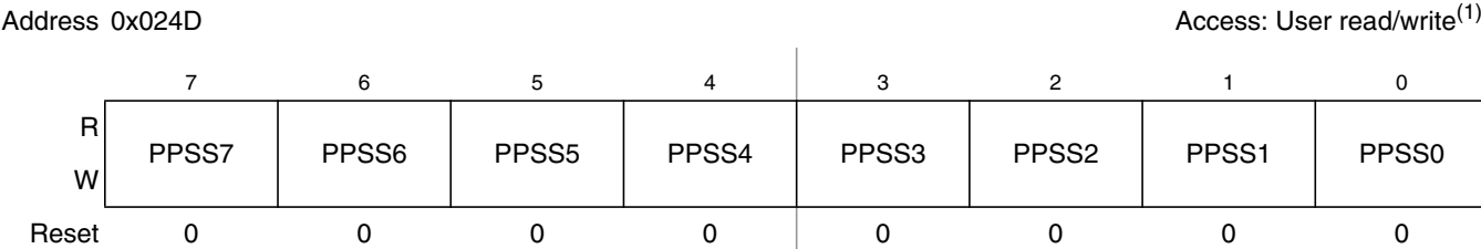
Figure 2-32. Port S Polarity Select Register (PPSS)
