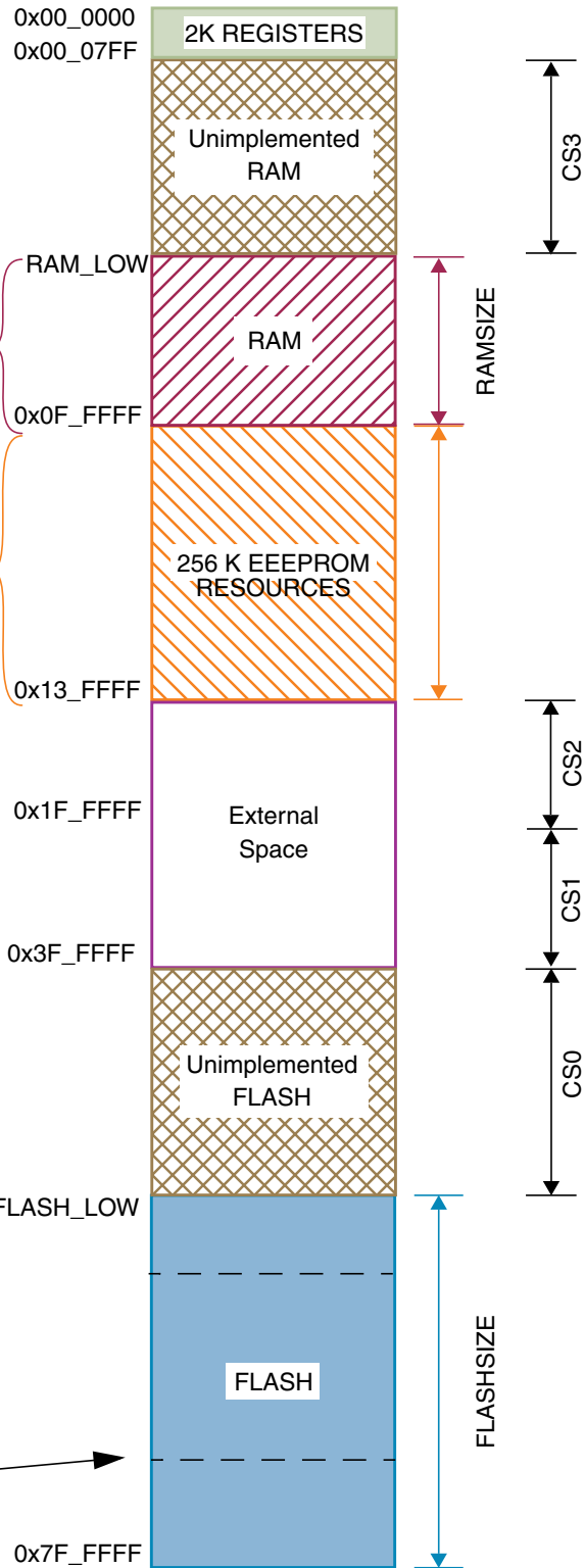
Figure 1-2. MC9S12XE100 Global Memory Map
