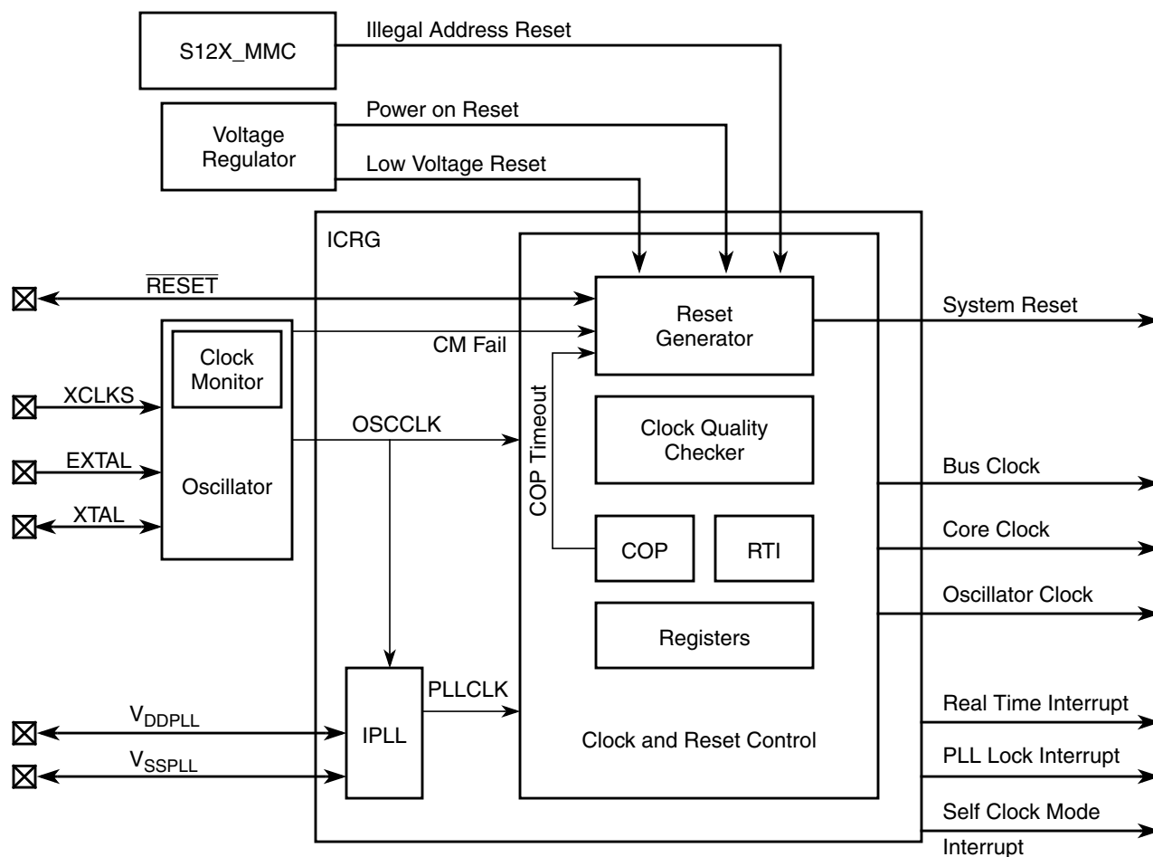
Figure 11-1. Block diagram of S12XECRG
