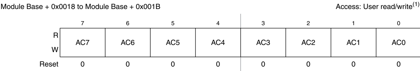
Figure 16-21. MSCAN Identifier Acceptance Registers (Second Bank) — CANIDAR4–CANIDAR7
