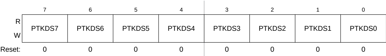
Figure 6-64. Drive Strength Selection for Port K Register (PTKDS)
