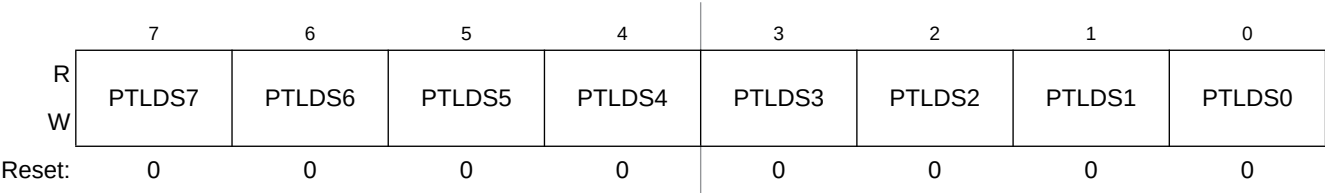
Figure 6-69. Drive Strength Selection for Port L Register (PTLDS)
