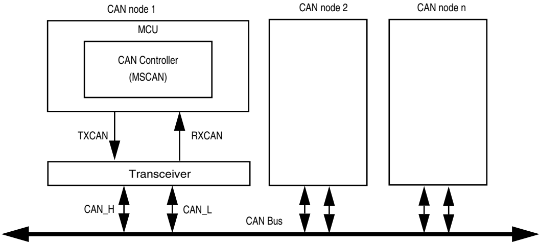
Figure 12-3. CAN System
