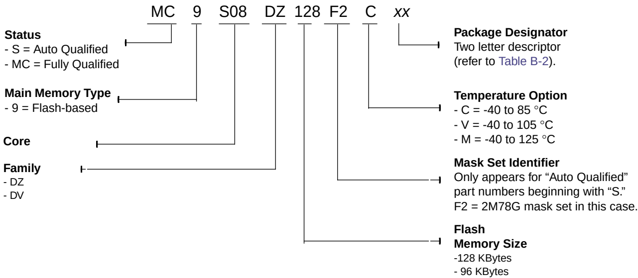
Figure 18-18. Device Numbering Scheme
