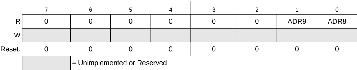
Figure 9-5. Data Result High Register (ADCRH)
