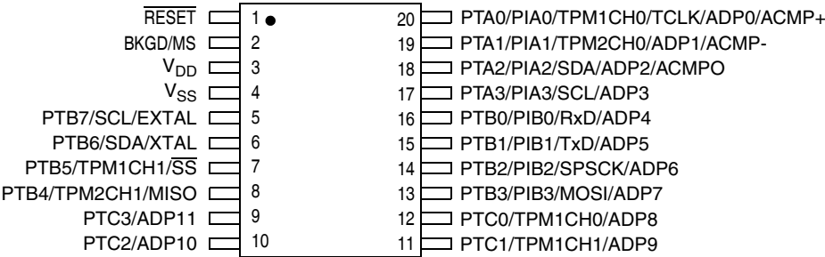
Figure 2-1. 20-Pin TSSOP
