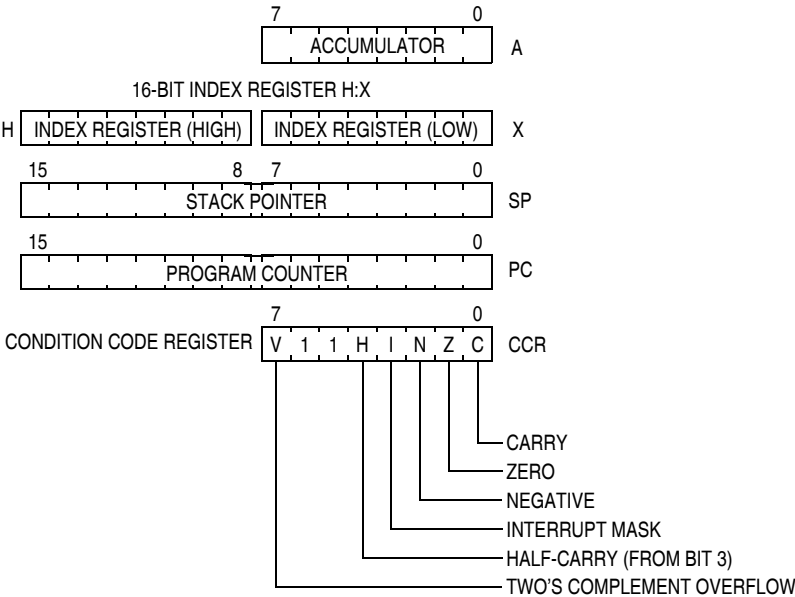
Figure 7-1. CPU Registers
