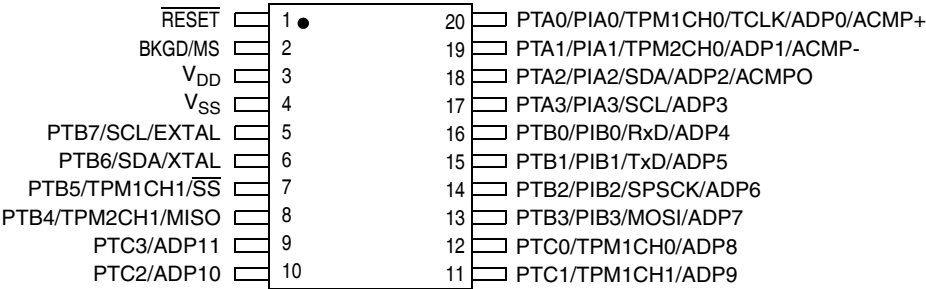
Figure 2-1. 20-Pin TSSOP
